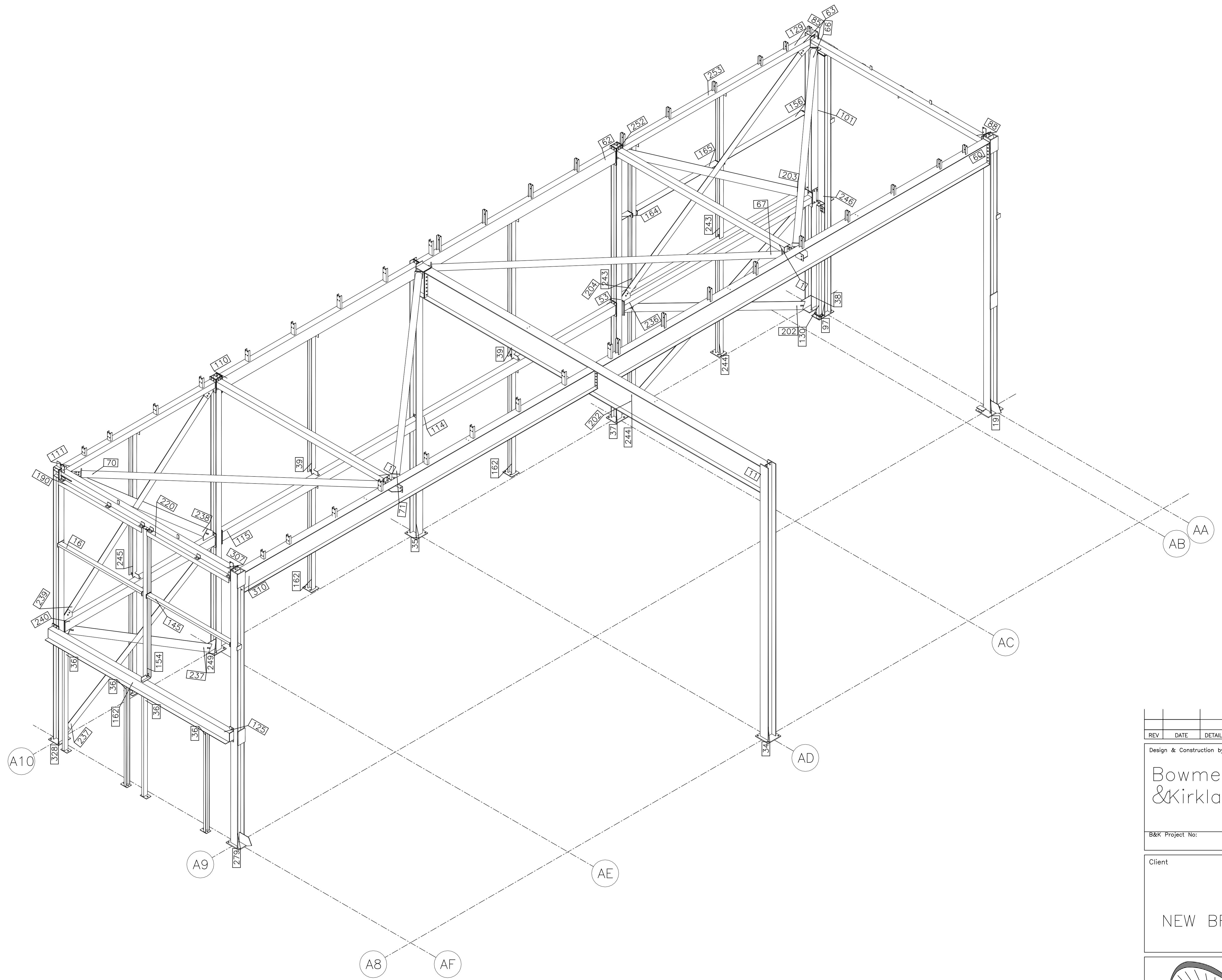
3-D MARKING VIEW LOT "1"
